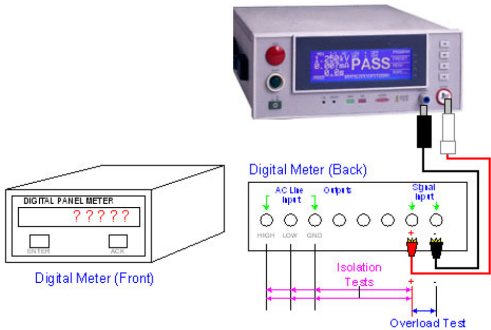
Figure 1: Test Setup with 19070 AC/DC/IR Hipot Tester
